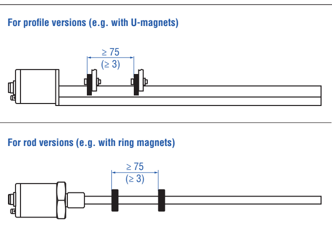
Fig. 45: Minimum distance between magnets for differentiation measurement (RP, RH, RD4, RF), example U-magnets (top) and ring magnets (bottom)
