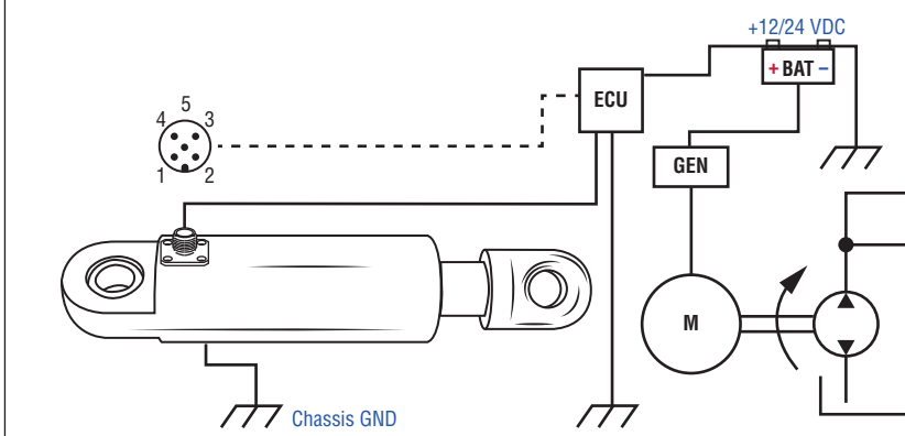
Fig. 9: Connection schematics
